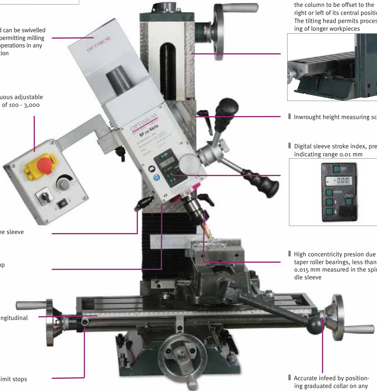
BF 20 Vario - illustration with optional collet holder, milling cutter and machine vice
